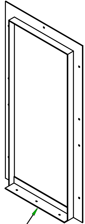
Step over frame (inside view of door frame)
